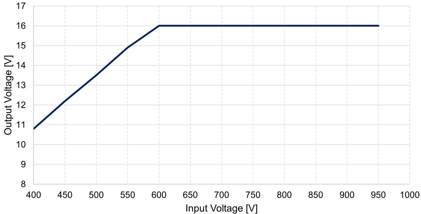
Vout vs Vin [V]/ Turns Ratio=17 PSFB-CDR topology, at Nominal Power limit
