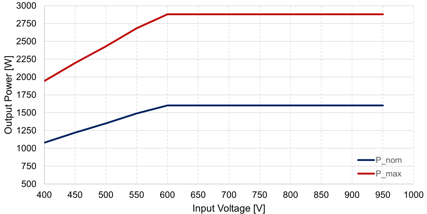
Pout [W] vs Vin [V]/ Turns Ratio=17 PSFB-CDR topology, at Nominal Input Voltage
