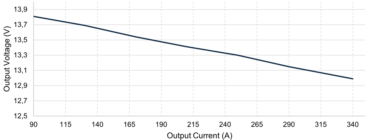
Voltage droop ( V_{out} vs I_{out} ) in dual rail operation
