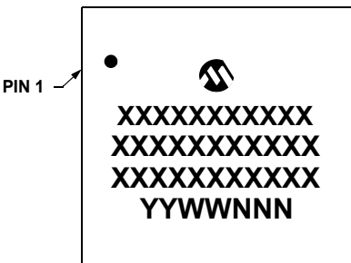
64-Lead VQFN (8x8 mm)
