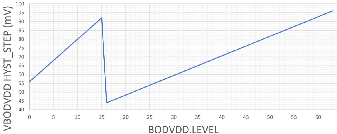
VBODVDD HYST_STEP (mV) versus BODVDD.LEVEL
