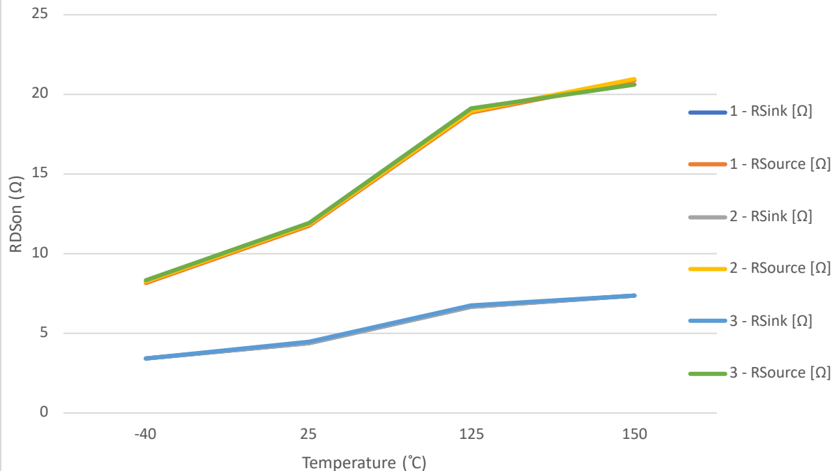
GDU LS Source/Sink Resistance ( R_{Source}/R_{Sink} ) vs. Temperature (IGLx = -100 mA, GDU = 1, 2, 3)
