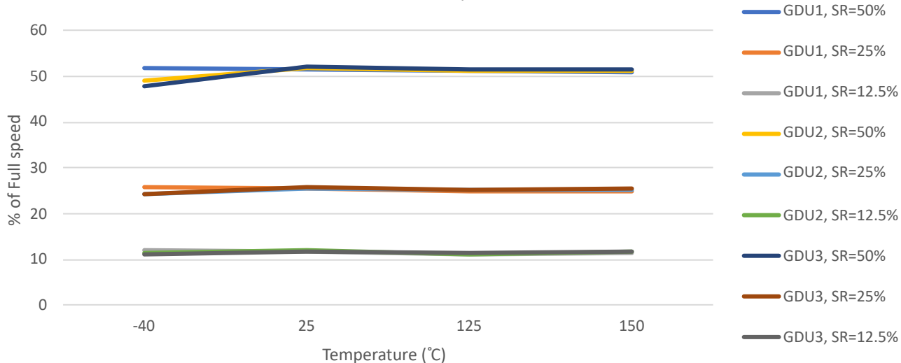
Low-Side Slew Rate Control vs. Temperature (LSSRC = 0, 1, 2, 3, GDU = 1, 2, 3)
