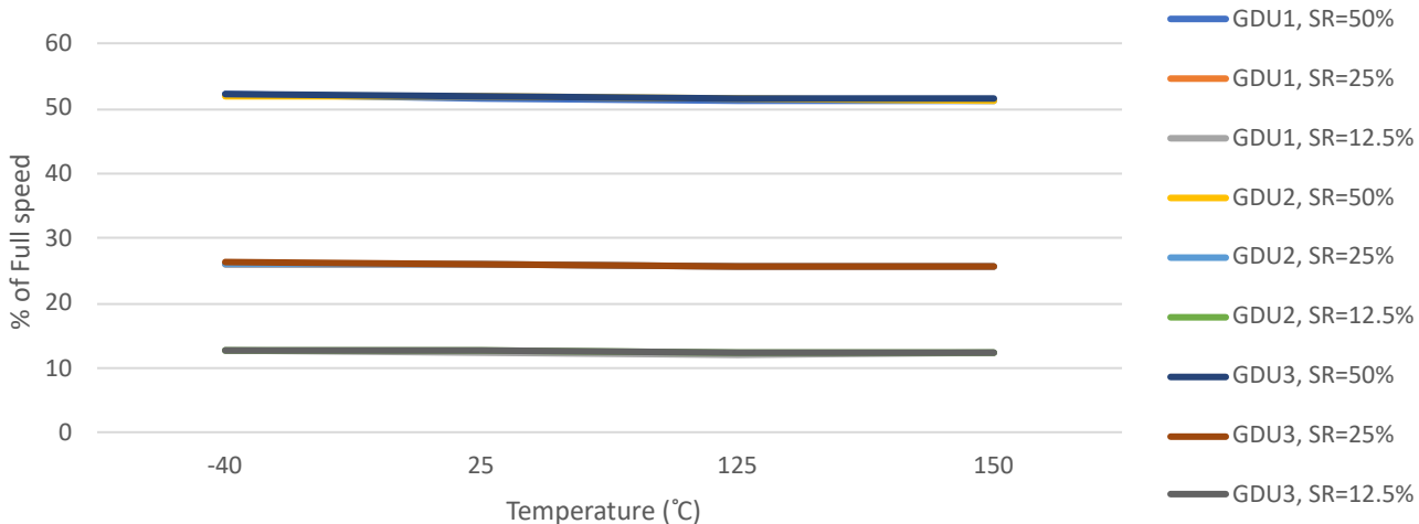
High-Side Slew Rate Control vs. Temperature (HSSRC = 0, 1, 2, 3, GDU = 1, 2, 3)
