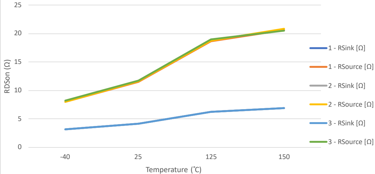
GDU HS Source/Sink Resistance ( R_{Source}/R_{Sink} ) vs. Temperature (IGHx = 100 mA, GDU = 1, 2, 3)
