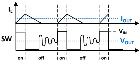
Discontinuous Inductor Current Mode
