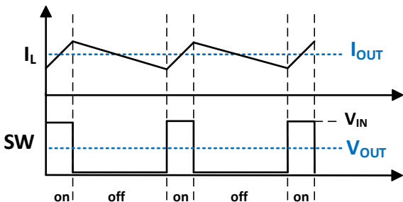
Continuous Inductor Current Mode
