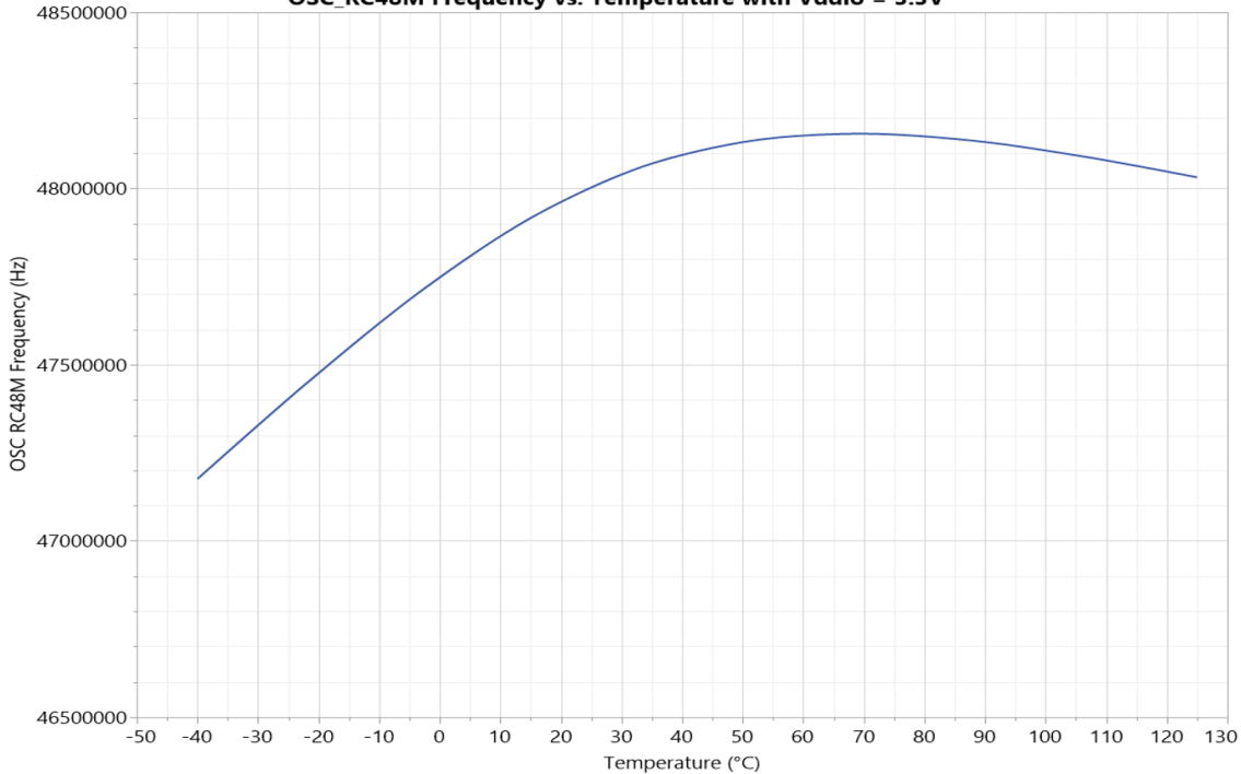
OSC_RC48M Frequency vs. Temperature with Vddio = 3.3V
