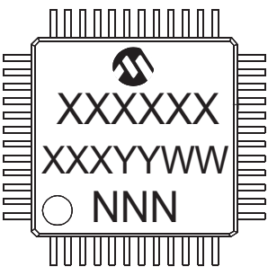
48-Lead TQFP (7x7 mm)
