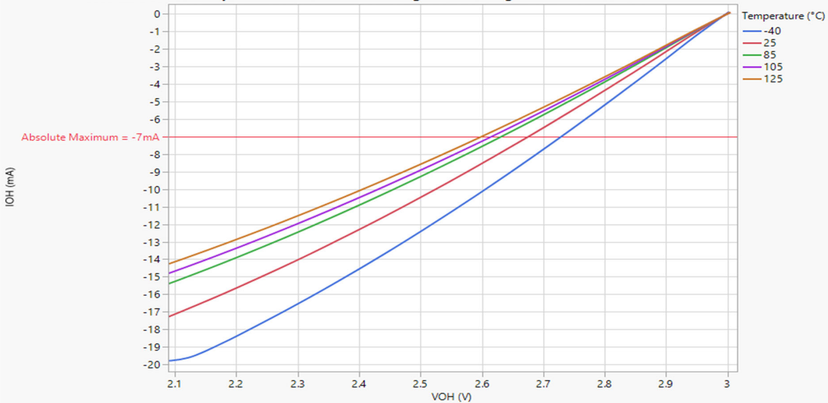
IOH vs. VOH vs. Temperature for Standard Pins High Drive Strength 1 with Vddio = 3V
