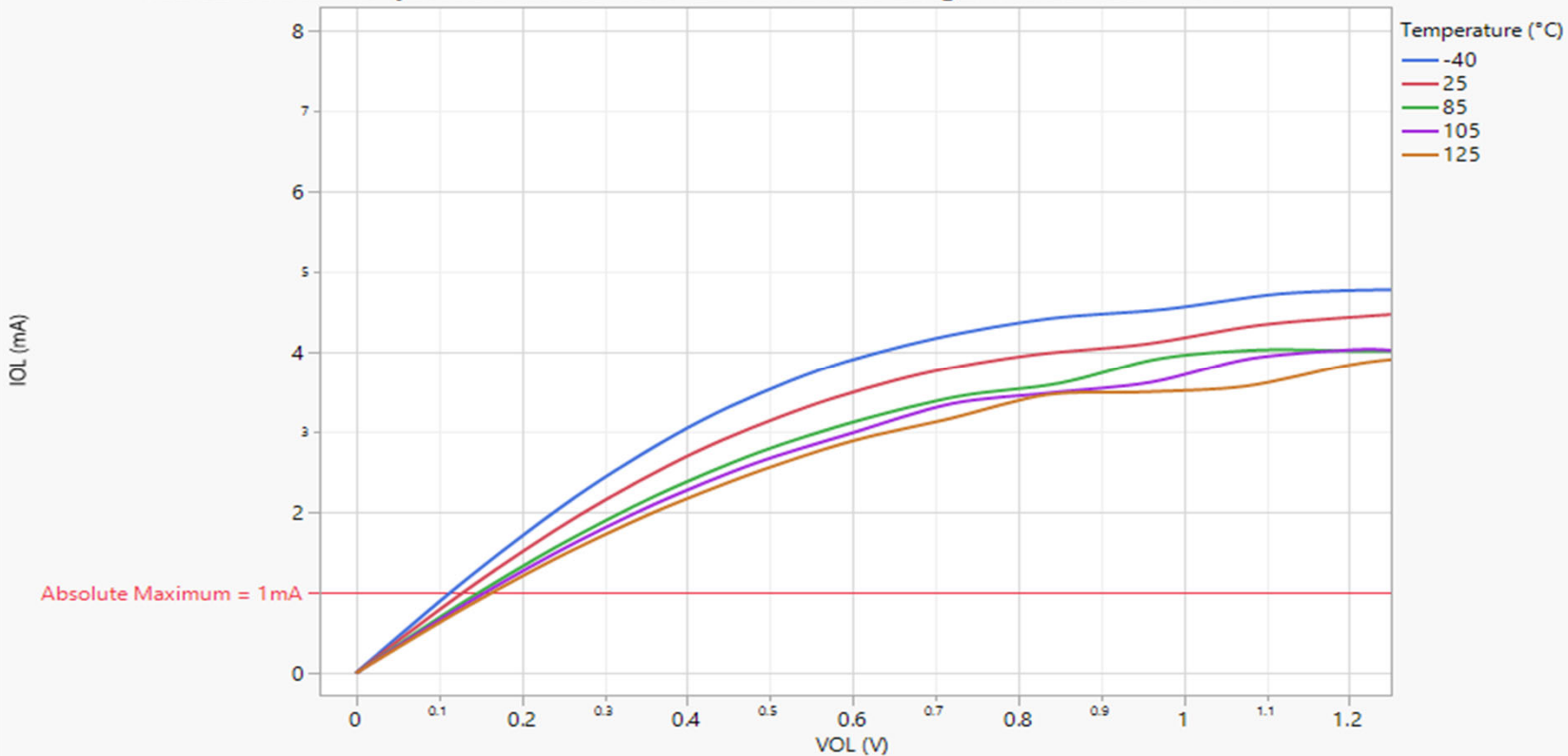
IOL vs. VOL vs. Temperature for Standard Pins Low Drive Strength 0 with Vddio = 1.6V
