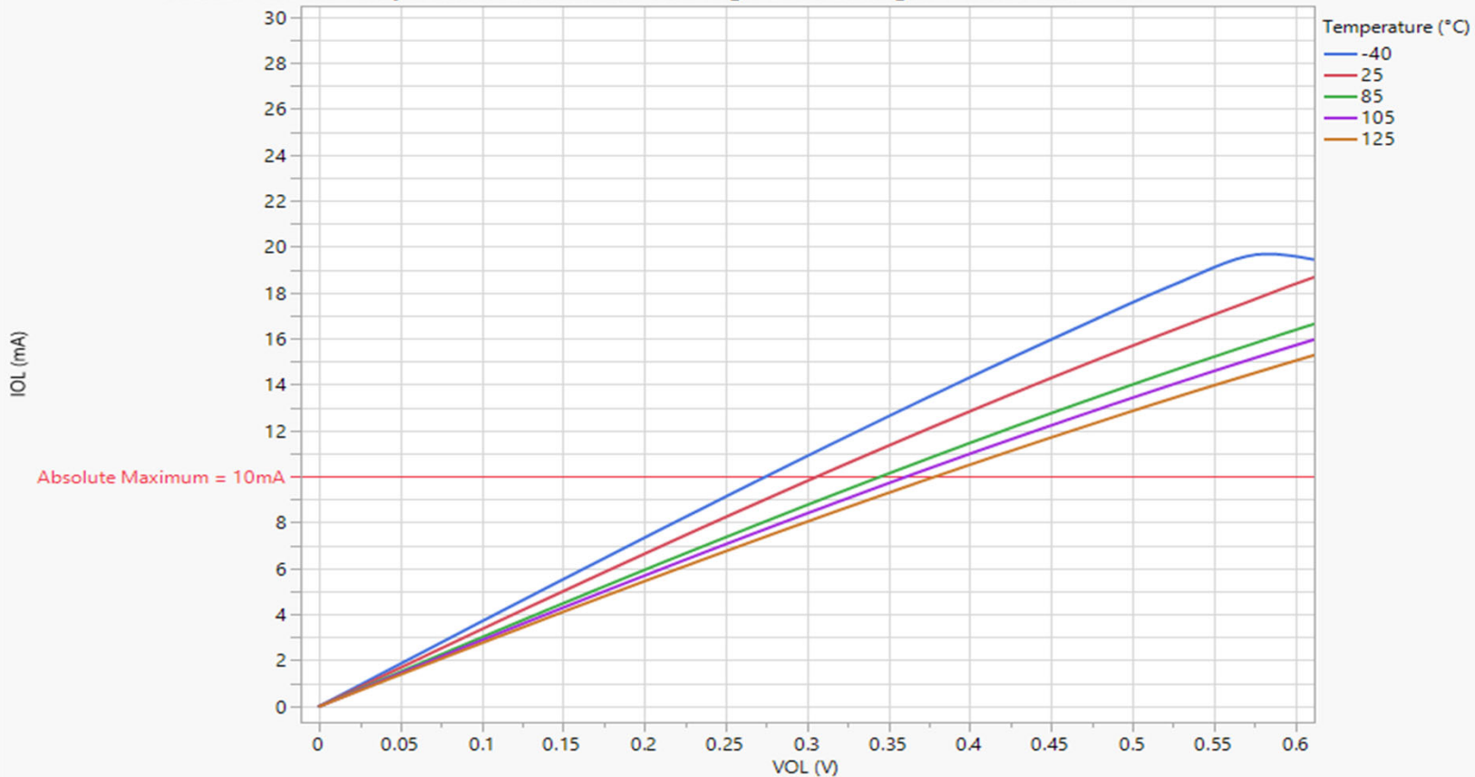
IOL vs. VOL for Standard Pins High Drive Strength 1 with Vddio = 3V
