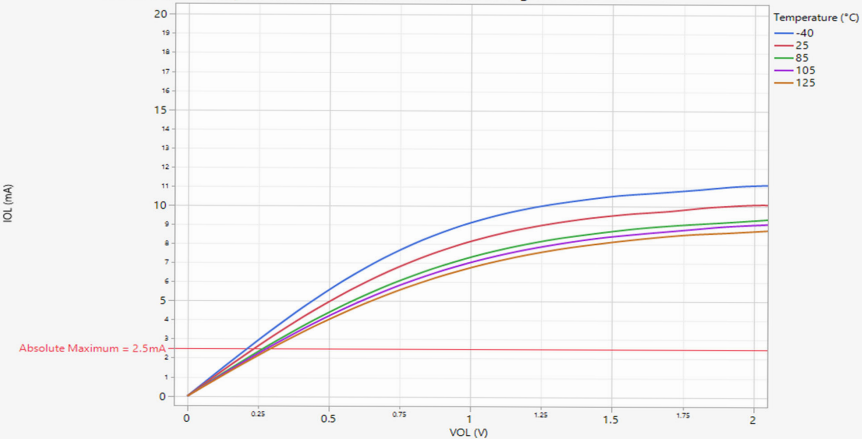
IOL vs. VOL vs. Temperature for Standard Pins Low Drive Strength 0 with Vddio = 3V
