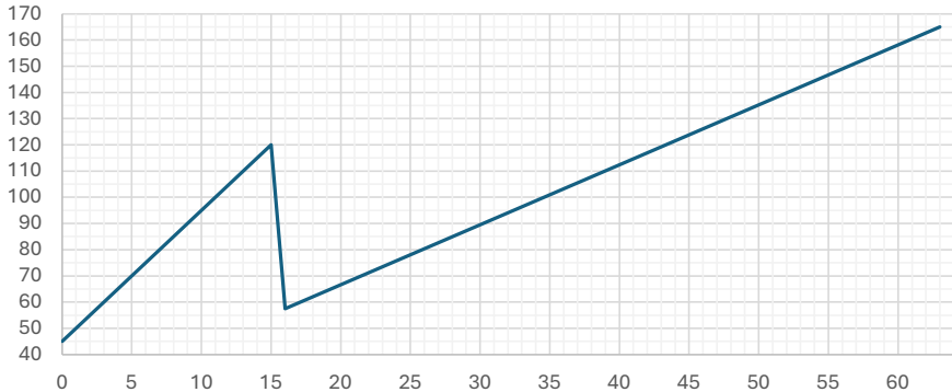
VBOD33 HYST_STEP (mV) versus BOD33.LEVEL
