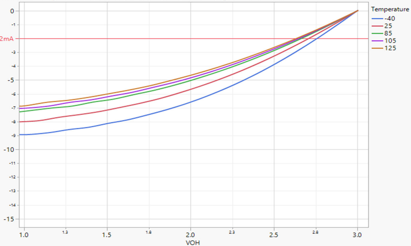
IOH vs. VOH vs. Temperature for Standard Pins Low Drive Strength 0 with Vddio = 3V
