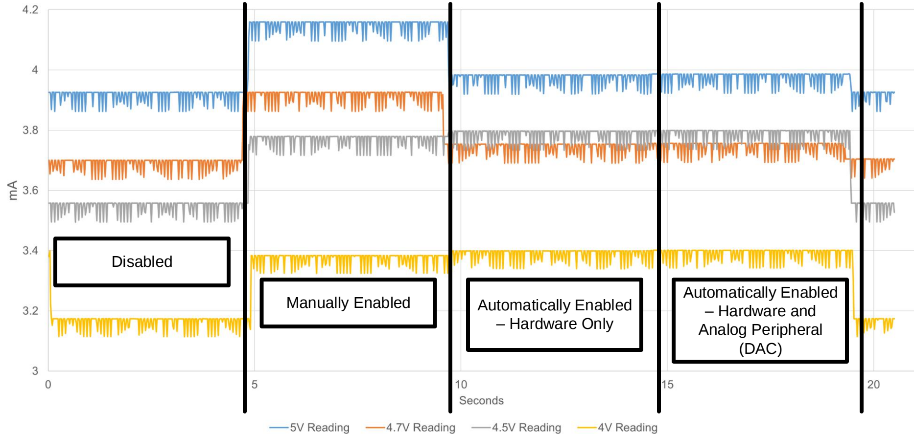
Current Used by the Charge Pump
