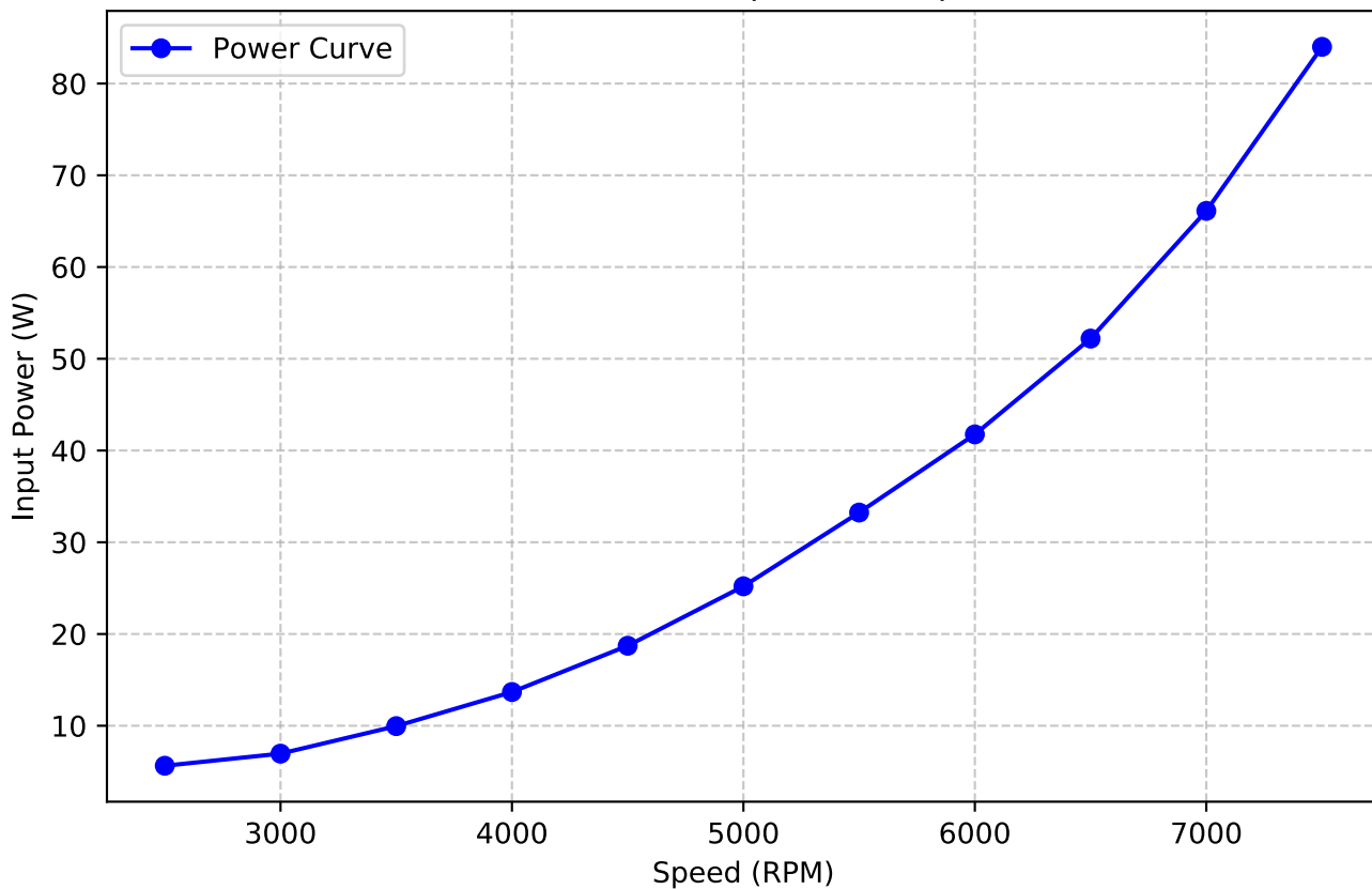
Motor Performance: Speed vs. Input Power
