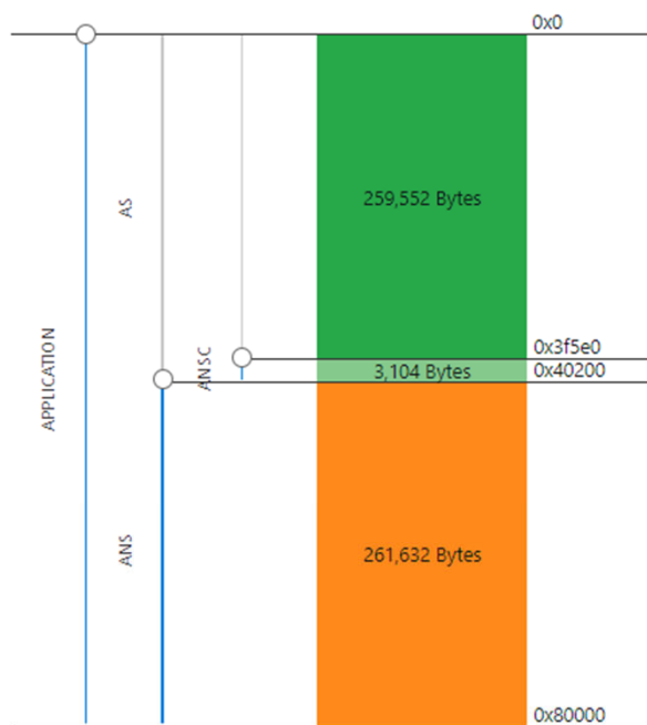
FLASH ( 524288 Bytes )
