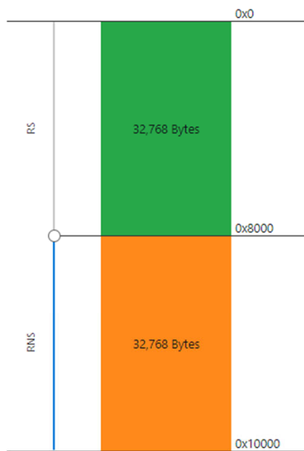
SRAM( 65536 Bytes )
