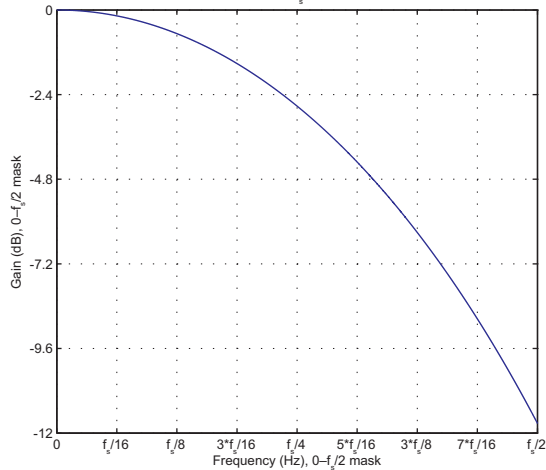
3rd order SINC filter 0-f_s/2 mask for OSR = 16
