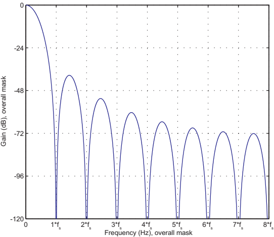
3rd order SINC filter overall mask for OSR = 16
