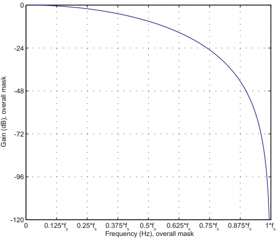
3rd order SINC filter overall mask for OSR = 2
