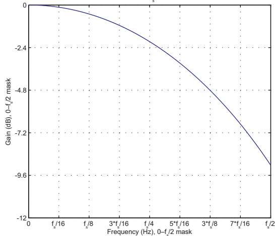
3rd order SINC filter 0-f_s/2 mask for OSR = 2
