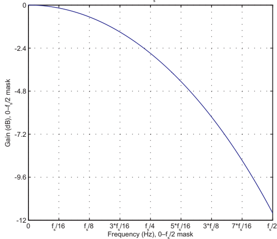
3rd order SINC filter 0-f_s/2 mask for OSR = 8
