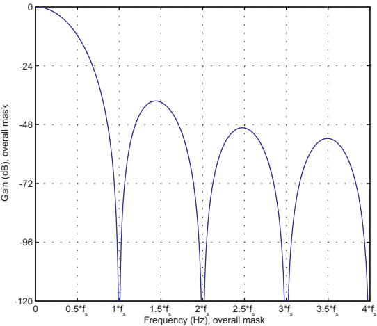
3rd order SINC filter overall mask for OSR = 8
