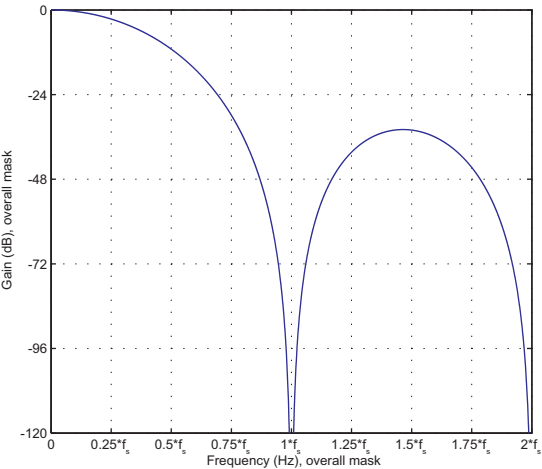
3rd order SINC filter overall mask for OSR = 4
