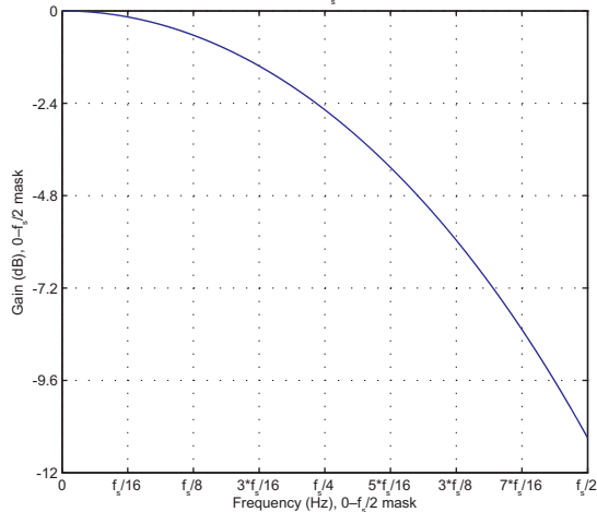
3rd order SINC filter 0-f_s/2 mask for OSR = 4
