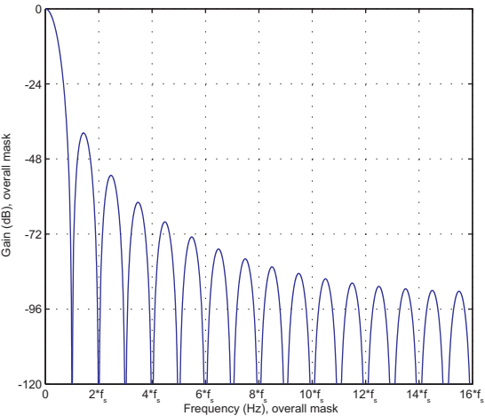
3rd order SINC filter overall mask for OSR = 32
