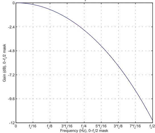
3rd order SINC filter 0-f_s/2 mask for OSR = 32
