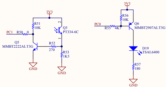
UART1 Opto-Port
