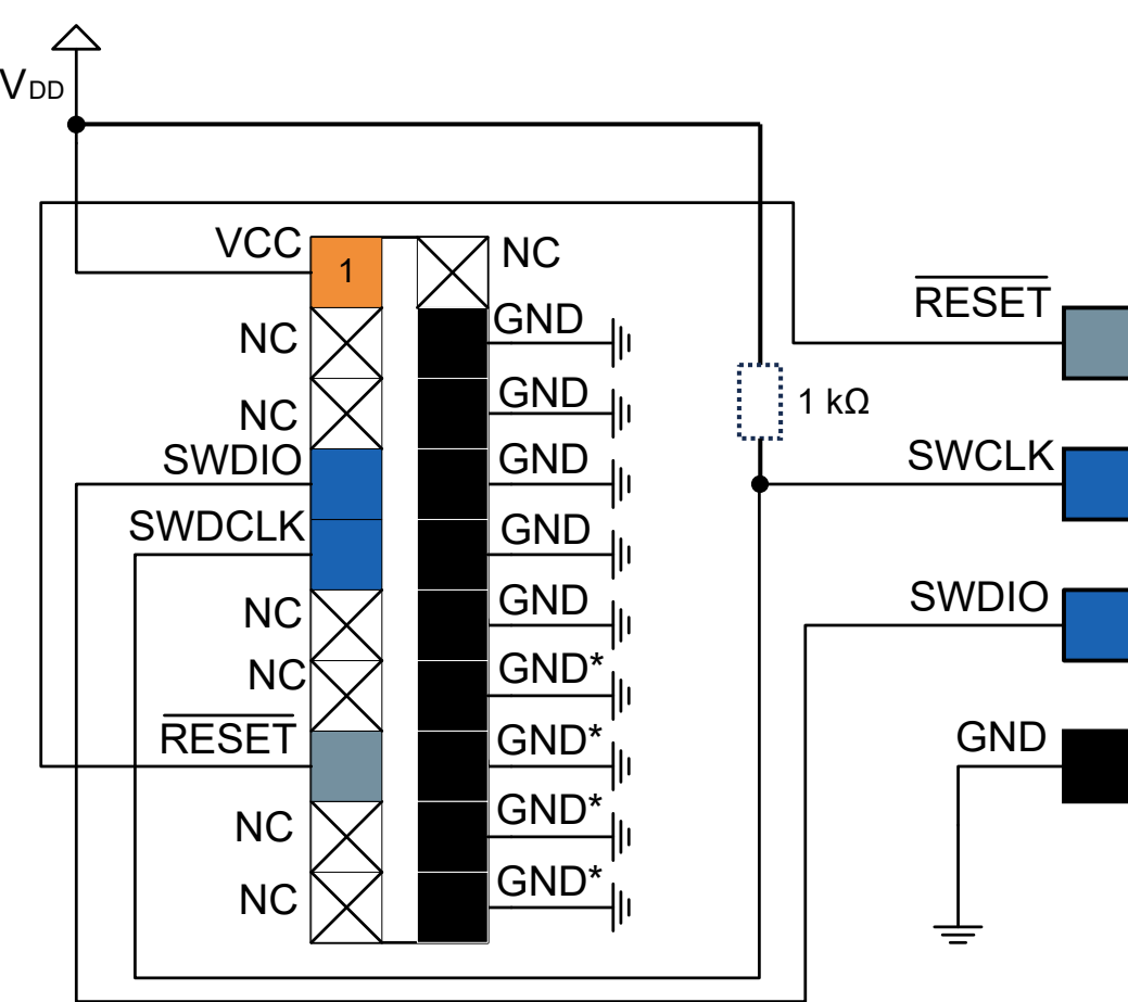
20-pin IDC JTAG Connector
