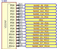
SAM9X75D2G-I/4TB-SL3
