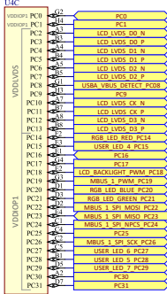
SAM9X75D2G-I/4TB-SL3
