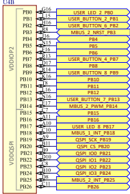
SAM9X75D2G-I/4TB-SL3
