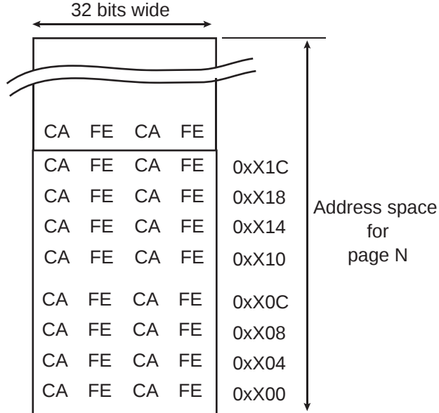
Before programming: unerased page in Flash array
