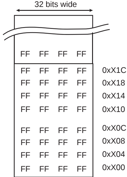
Step 1: Flash array after pages erase
