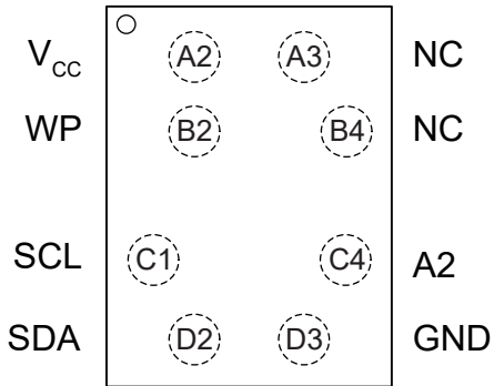
8-Ball WLCSP (Top View)
